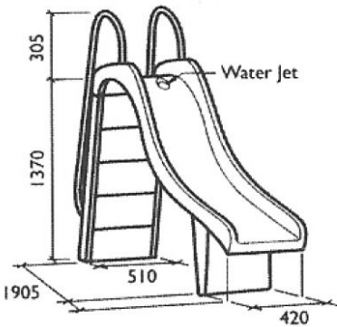
Straight Side Sketch
