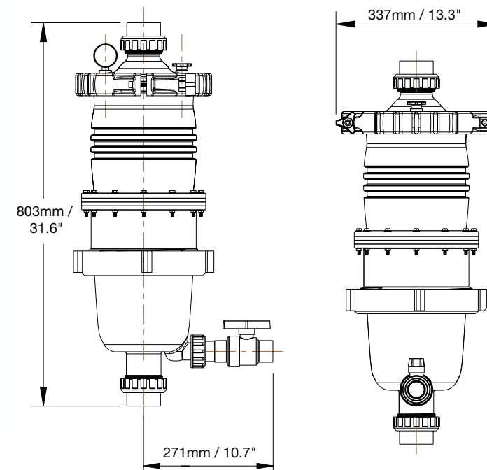
MultiCyclone 16 Plus
