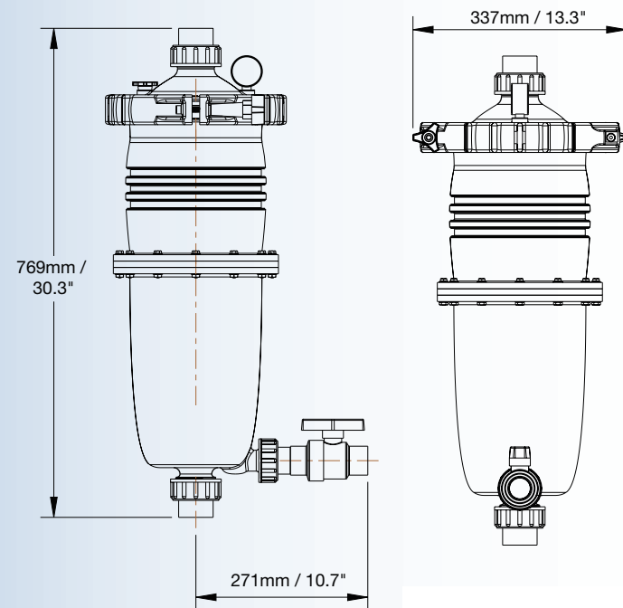
MultiCyclone 12 Plus
