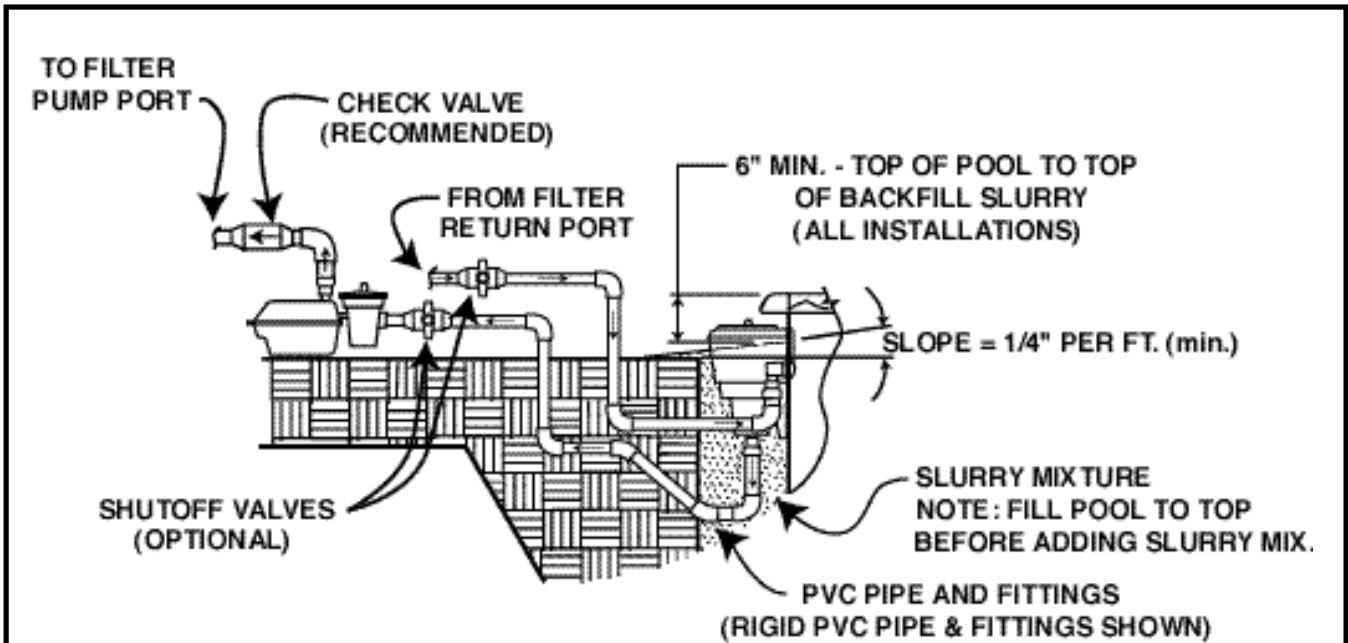
FIG. 4 - TYPICAL PLUMBING INSTALLATION
