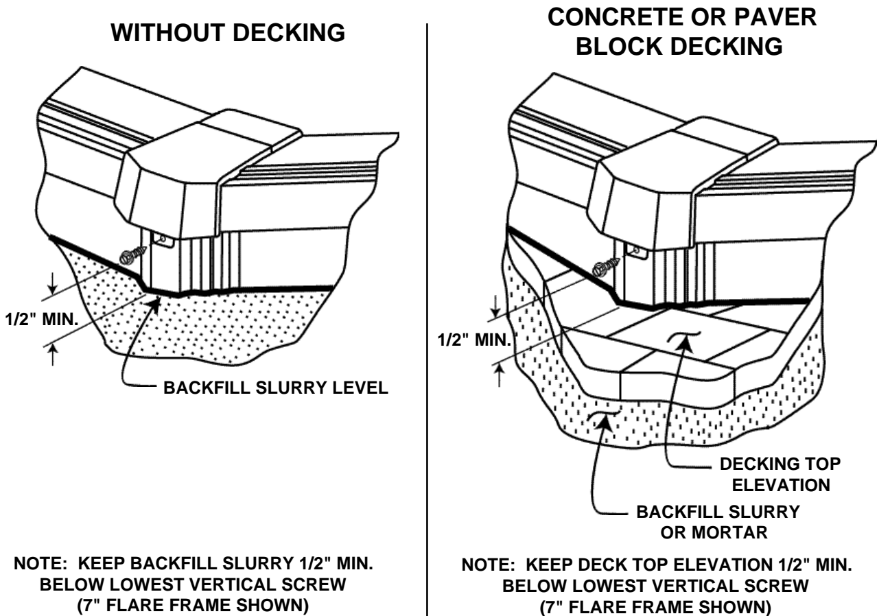
FIG. 5 - DECK ELEVATION
