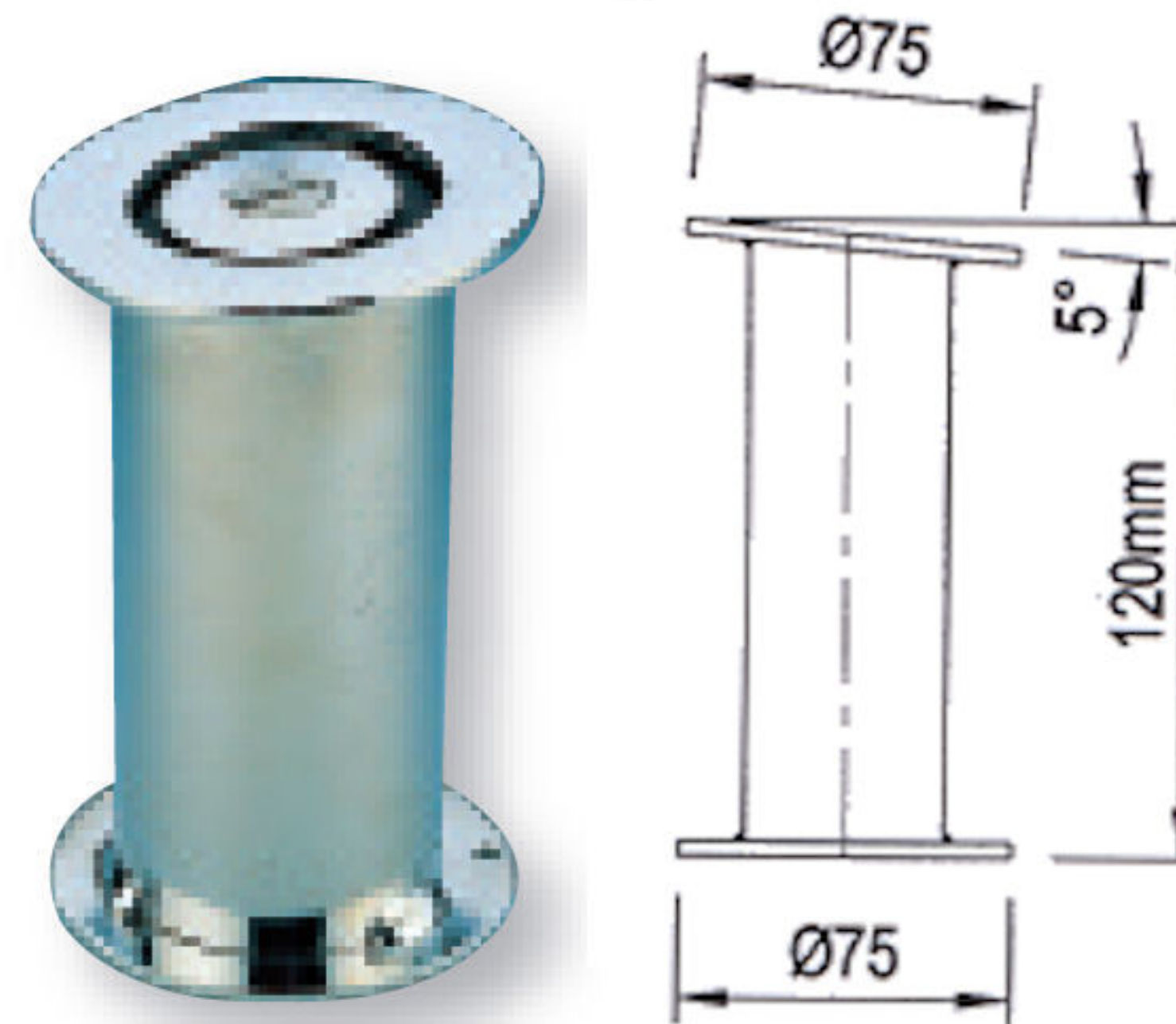
Inclined Anchor Fixing
