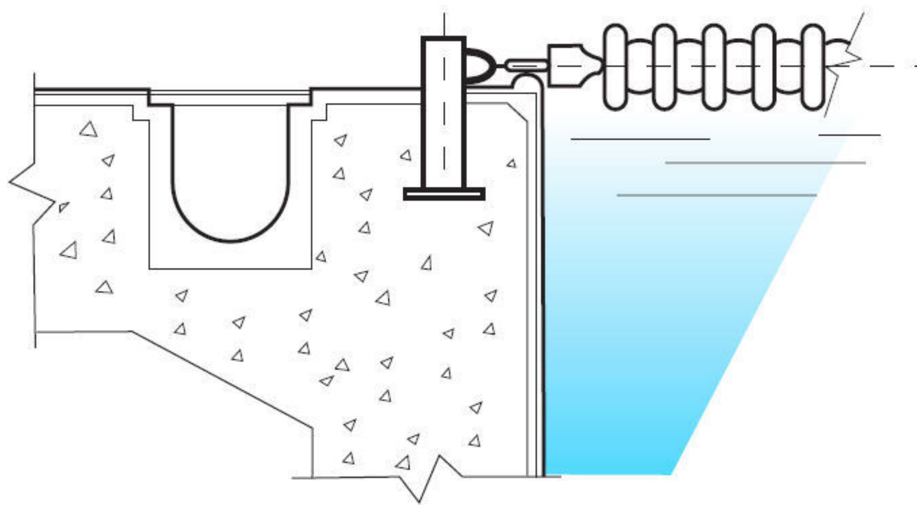
CEMLA43 CEMFLS Level Anchor Float Line Support
