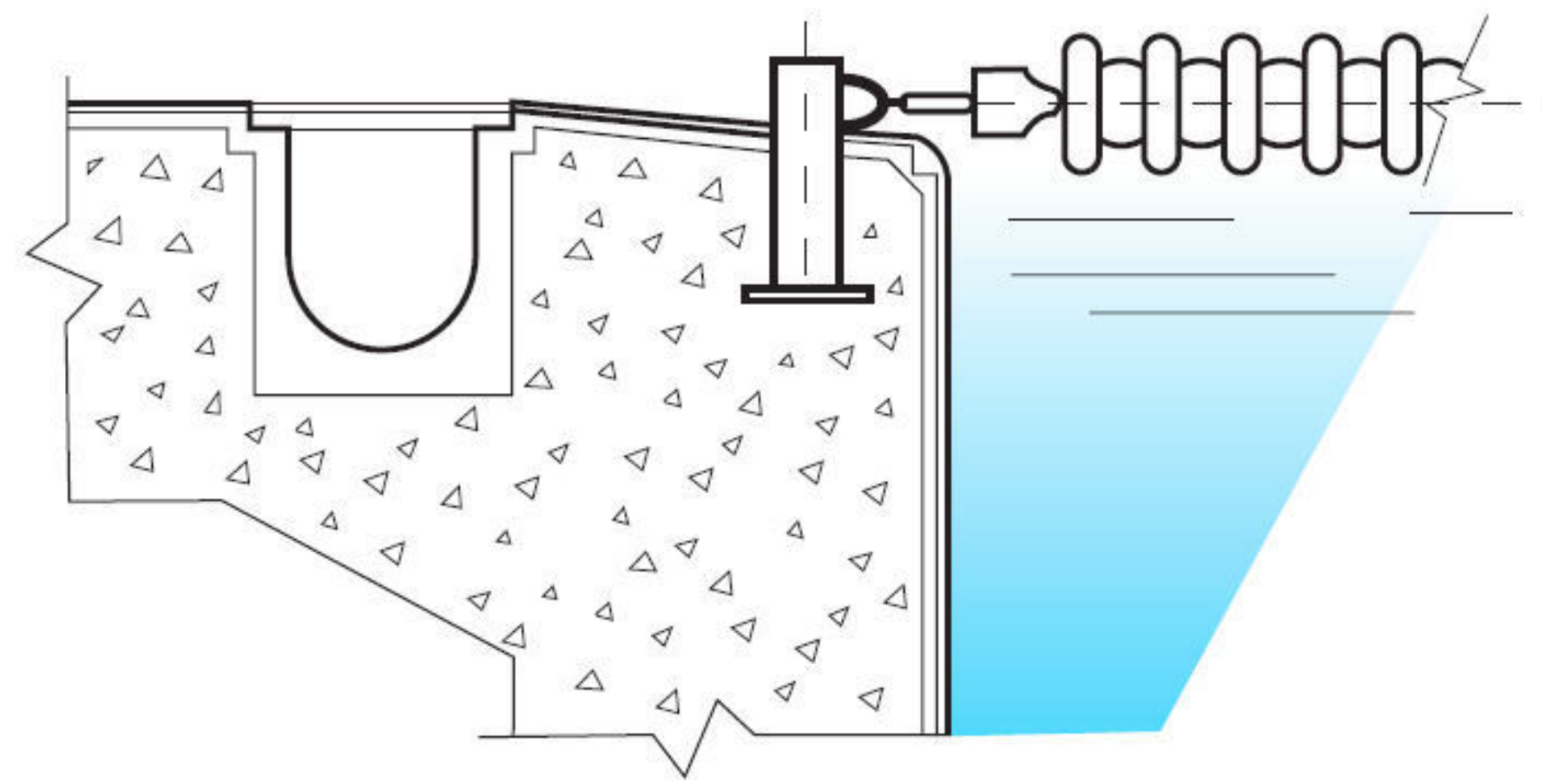
CEMIA43 CEMFLS Inclined Anchor Float Line Support
