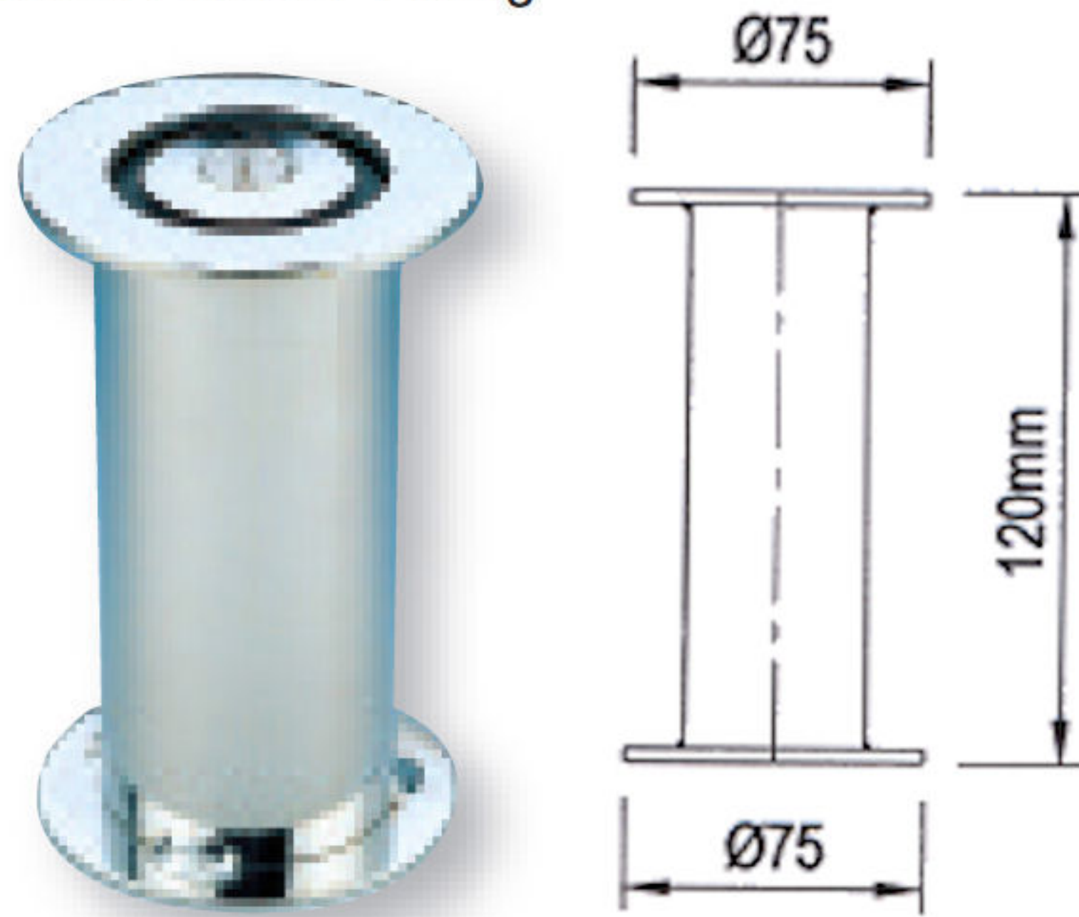
Level Anchor Fixing
