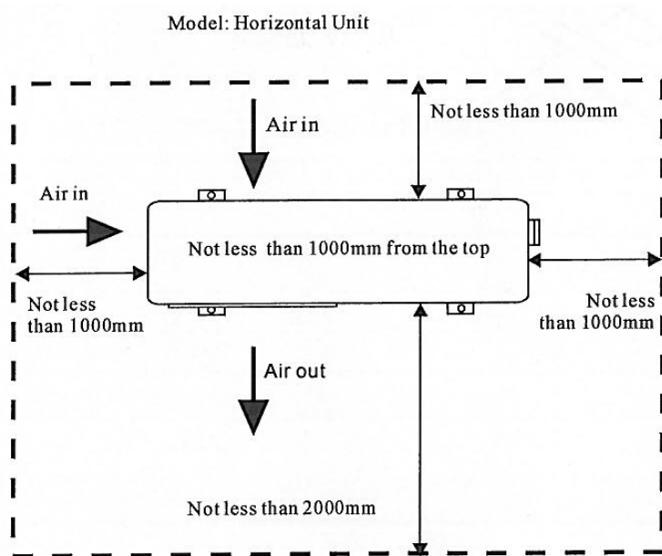
Free space requirement for the horizontal heat pump
