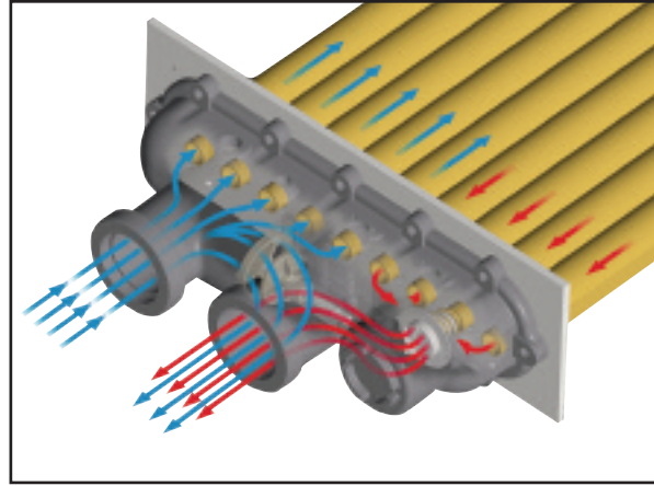
Pressure sensitive bypass and temperature sensitive throttle valve ensure trouble free operation.
