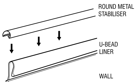
Installation detail of the u-bead liner.
