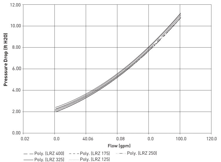
LRZ With a Polymer Header Models Loss Chart
